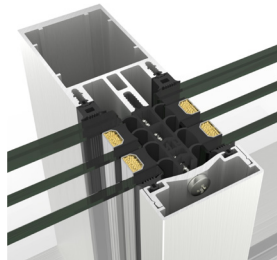
Mullion Detail
