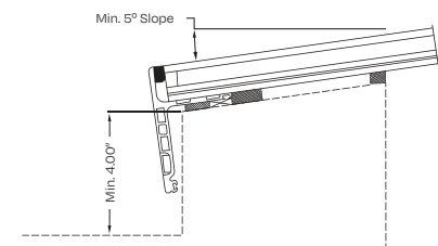
Detail View
