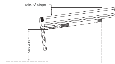
Detail View
