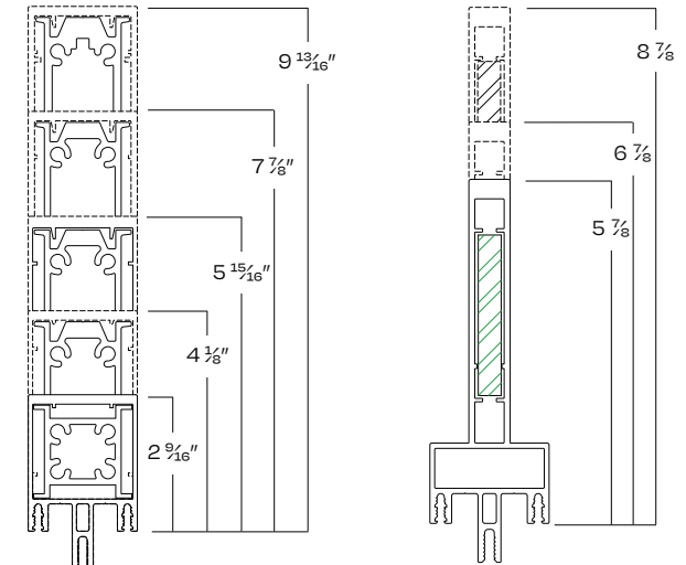
Box Mullion
